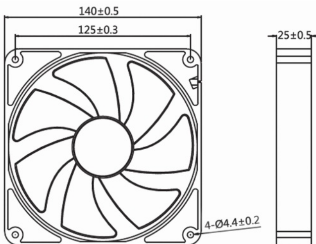
Dimensions Drawing
