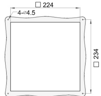
Mounting profile 安裝剖面 M9804
