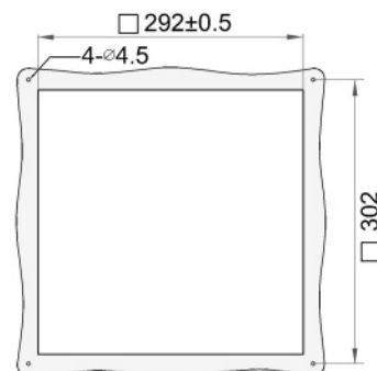
Mounting profile 安裝剖面 M9805
