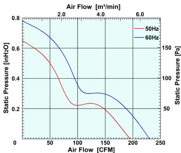
Air Flow &amp; Static Pressure Curve
