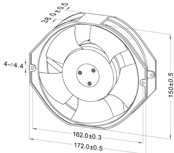
Dimensions Drawing
